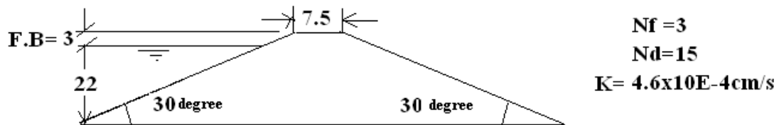
Fig.2 Q.3(a) OR All Dimensions are in m
