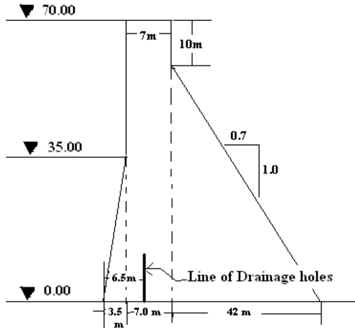
Fig.-1 Section of Gravity Dam Q-3(a)
